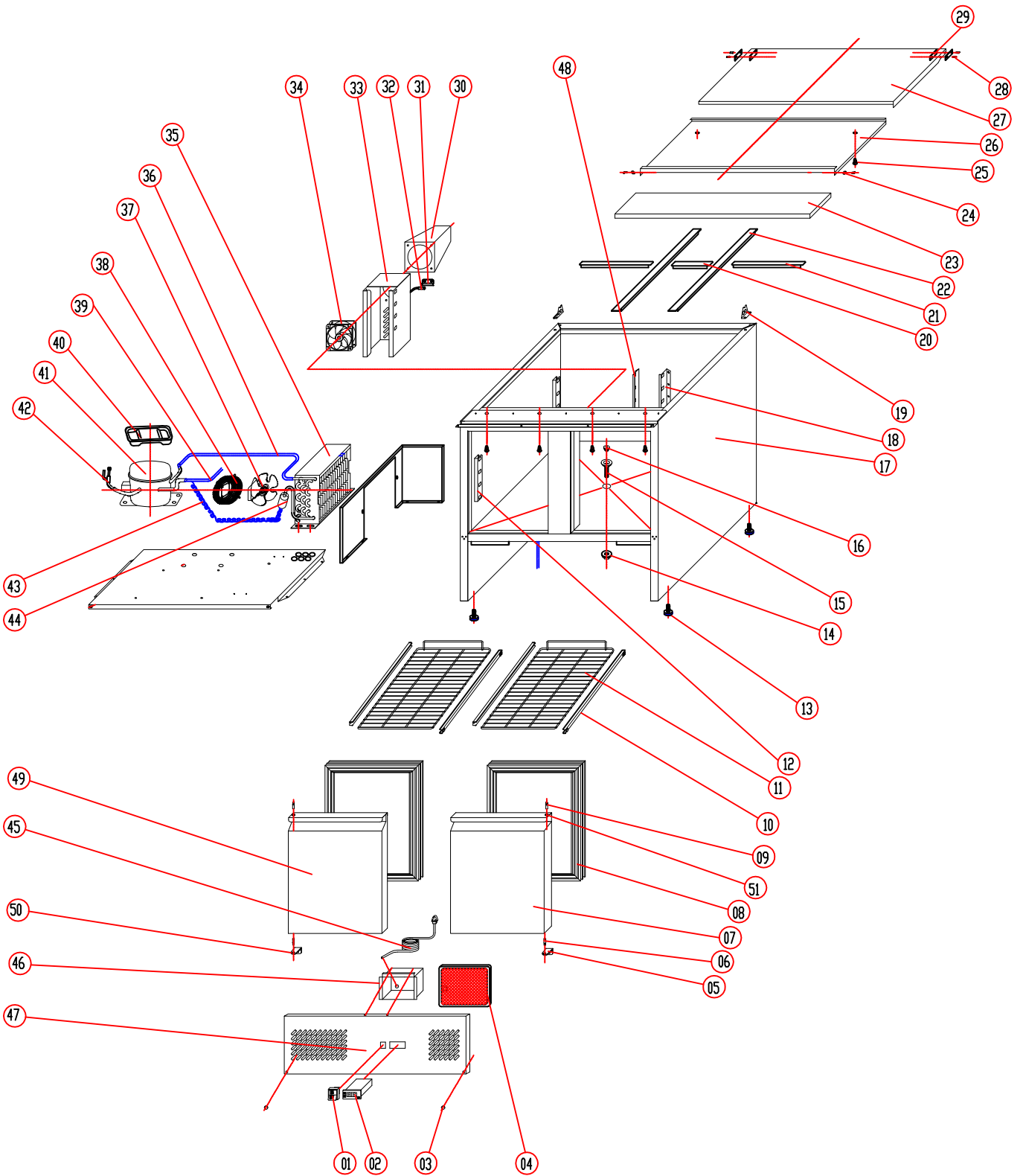
EXPLODED VIEW OF S900
